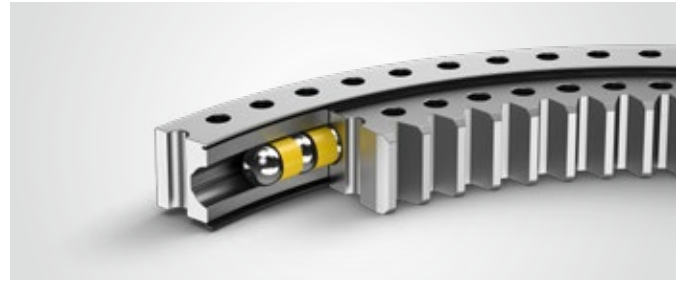
Single-row four-point bearings – with internal gear
