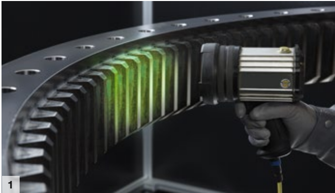
1 Magnetic particle inspection
