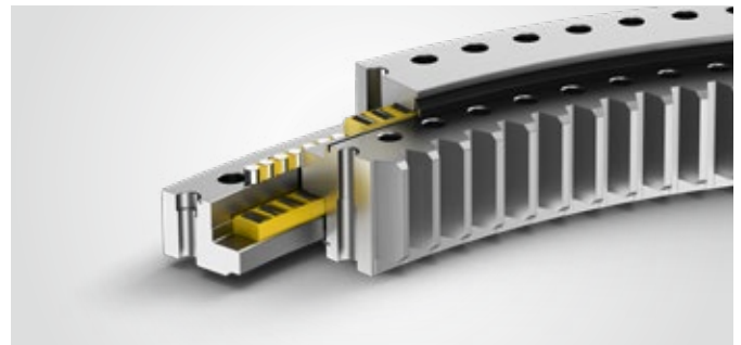
Triple-row roller bearings – with internal gear
