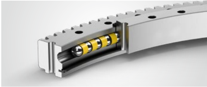
Single-row four-point bearings – with external gear
