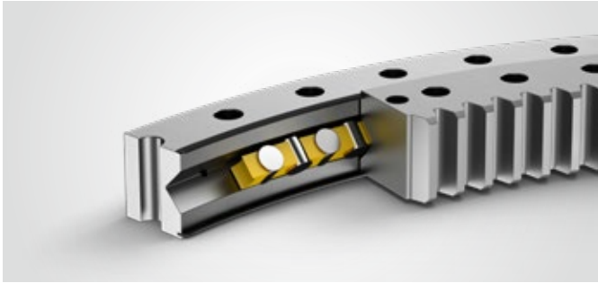
Cross roller bearings – with external gear/with internal gear/no gear
